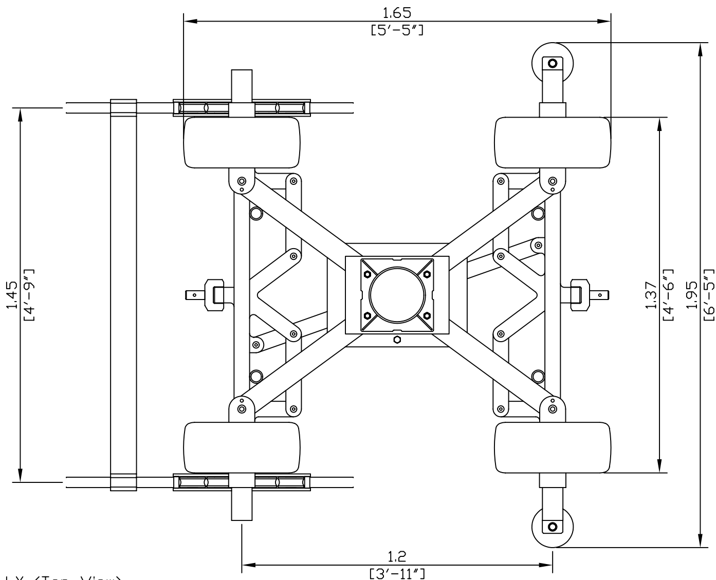
DOLLY (Top View)
