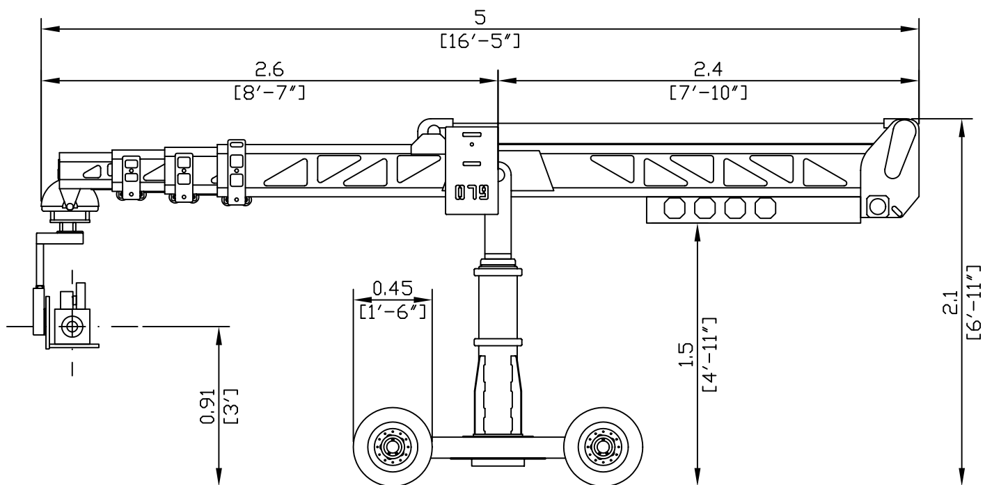
CRANE COMPACT (Side View)
