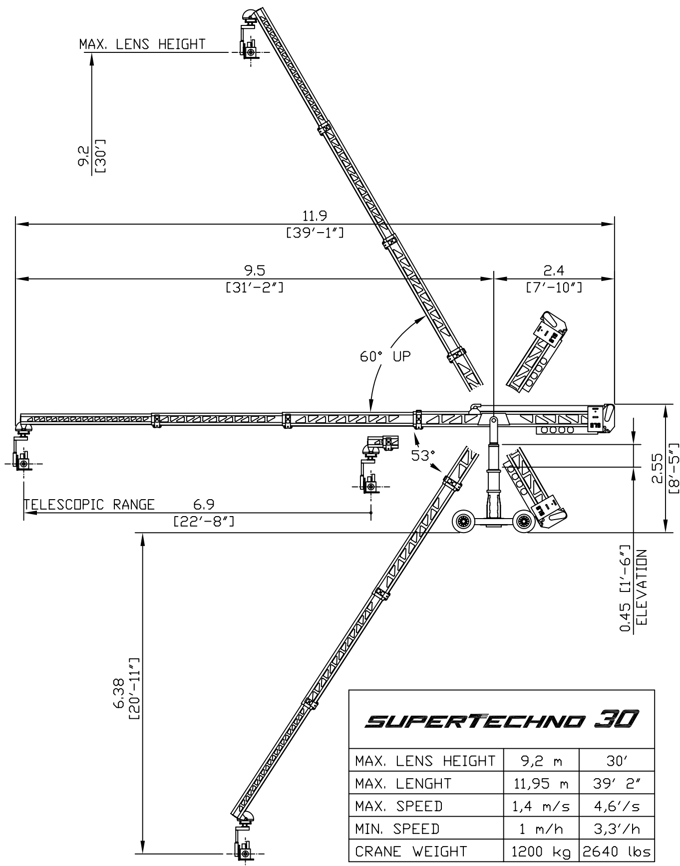
CRANE FULLY EXTENDED (Side View)
