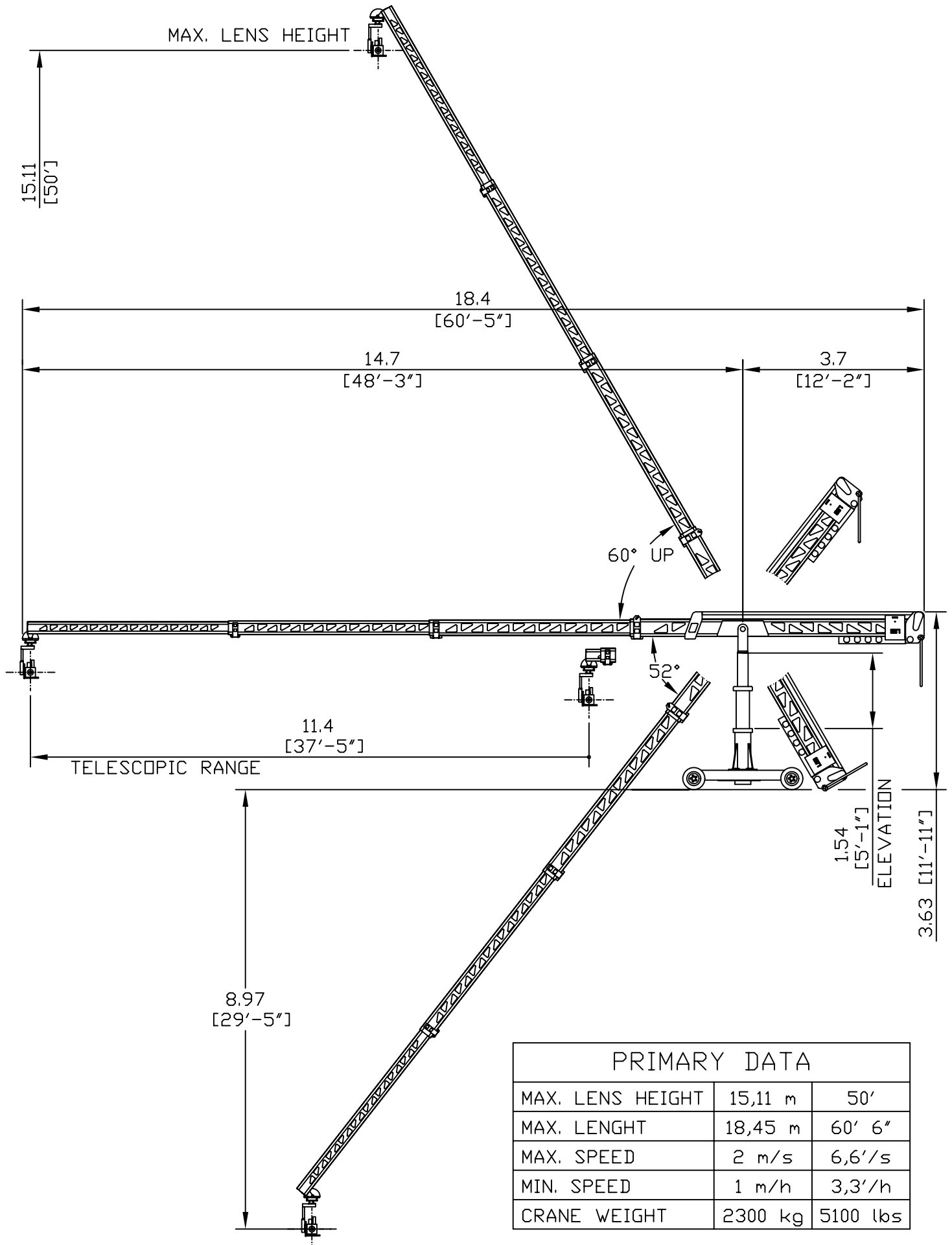
CRANE FULLY EXTENDED (Side View)
